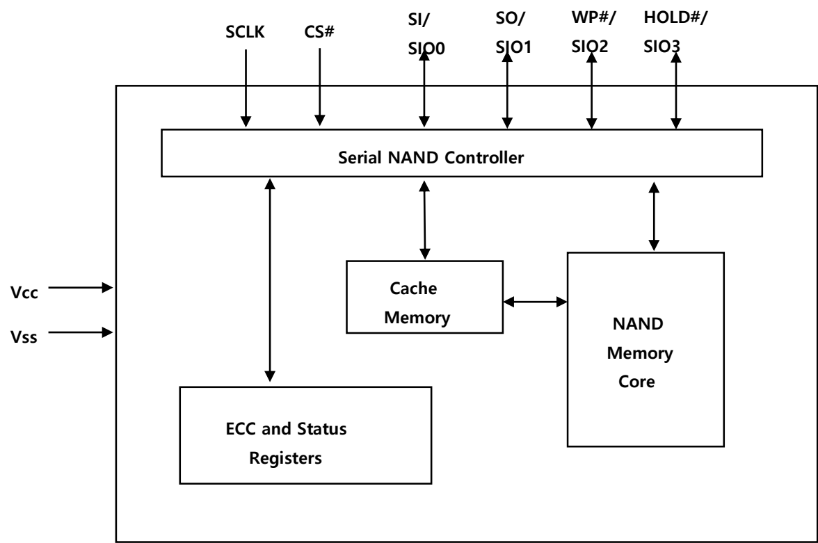
Figure 1.2 Block Description
