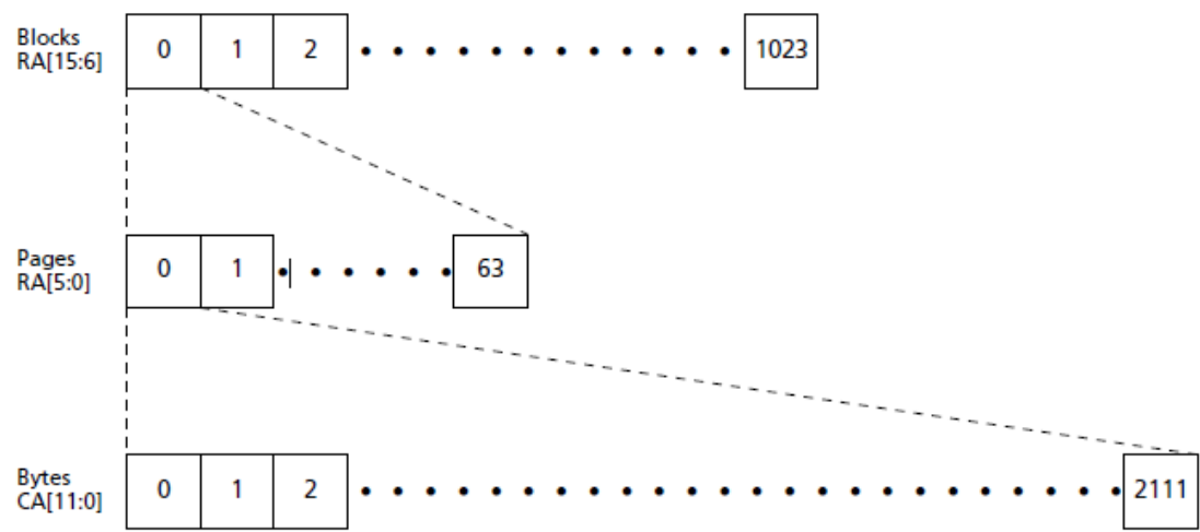
Figure 1.3 Address Map
