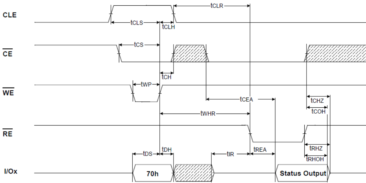
Figure 8 : Status Read Cycle
