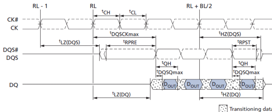
Figure 4 : READ Output Timing – tDQSCK (MAX)
