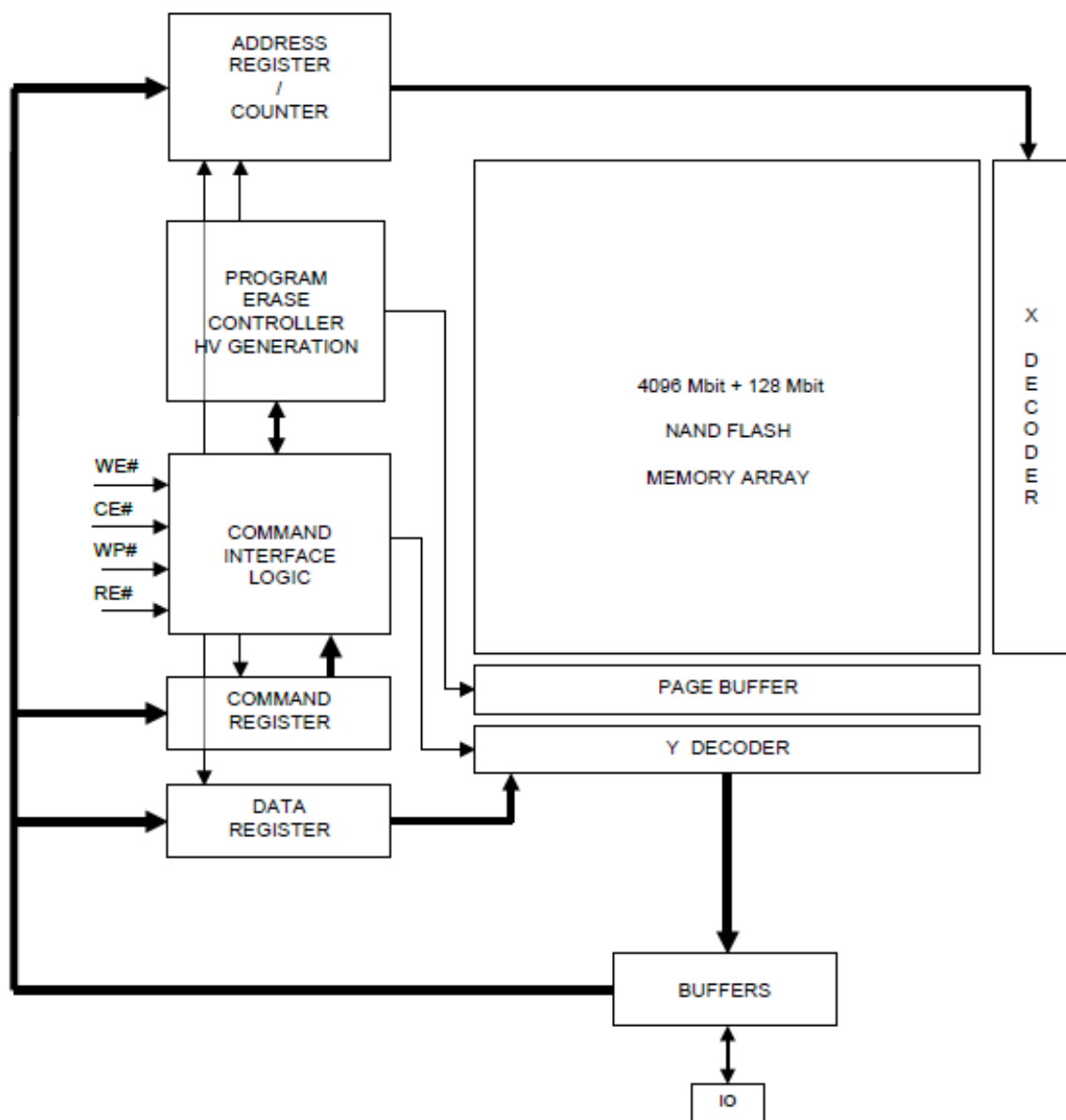
Figure 2 : block description
