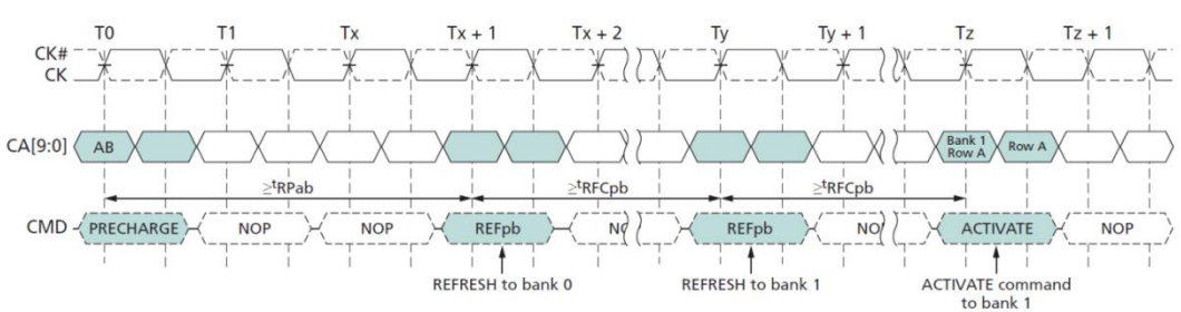
Figure 34 Per-Bank REFRESH Operation
