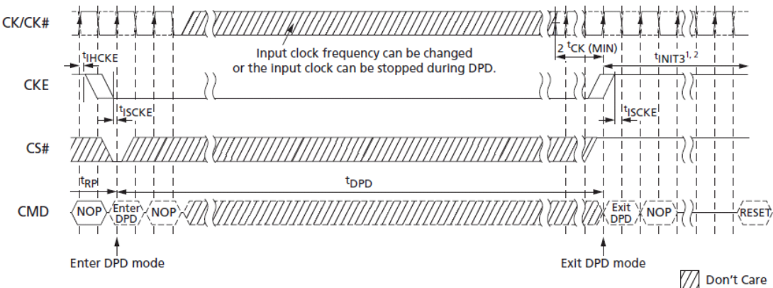
Figure 55: Deep Power-Down Entry and Exit Timing
