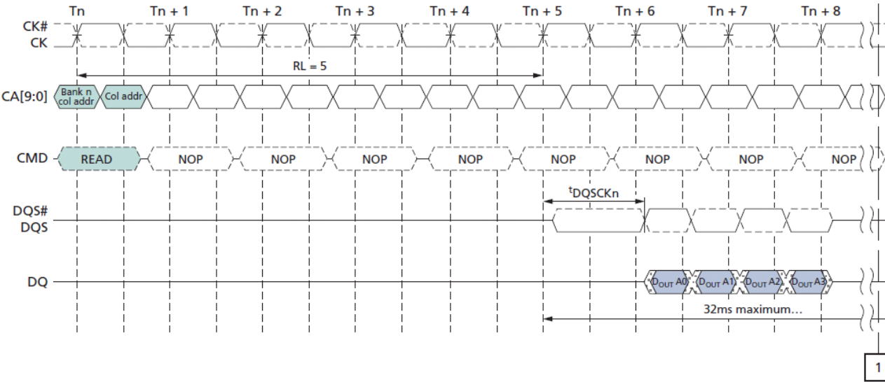
Figure 8 : tDQSKDL Timing
