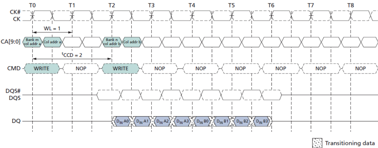
Figure 17 : Seamless Burst WRITE – WL = 1, BL = 4, tCCD = 2
