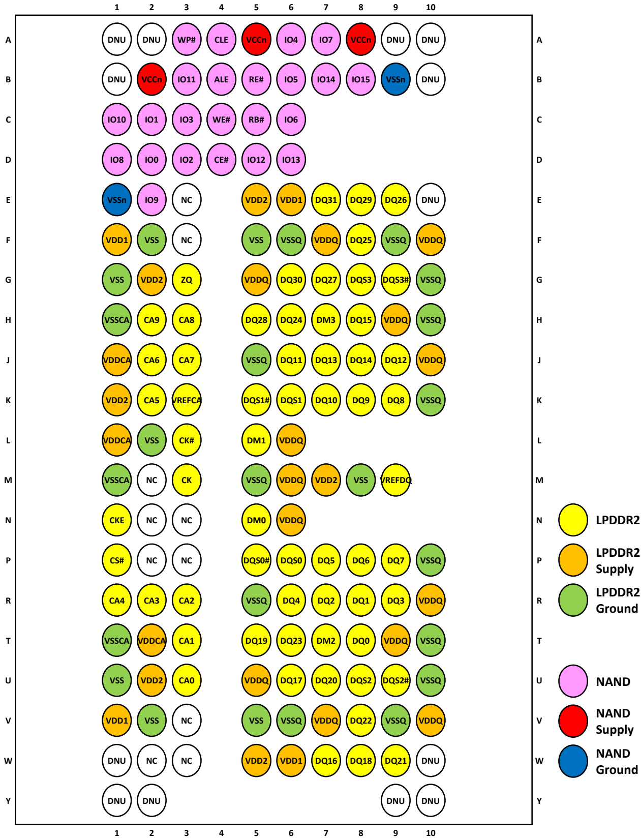
Pin Configuration – 162Ball MCP(X16/X32)
