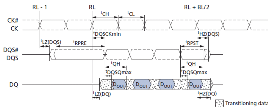
Figure 5 : READ Output Timing – tDQSCK (MIN)
