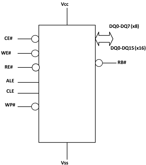
Figure 1: Logic Diagram
