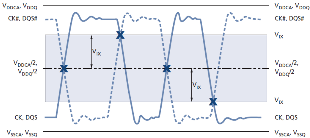
Figure 61: Vix Definition
