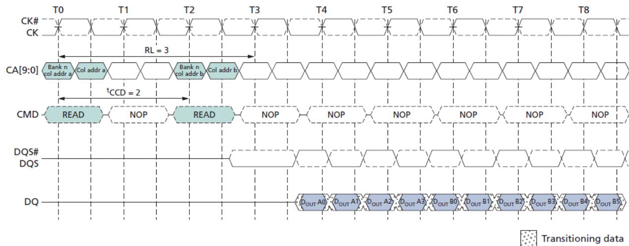
Figure 13: READ Burst Interrupt Example – RL = 3, BL = 8, tCCD = 2
