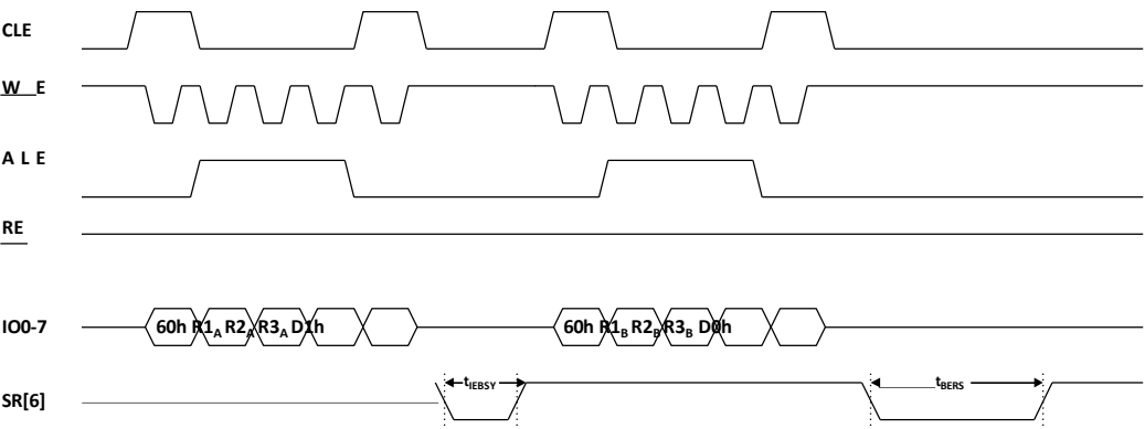
Figure 24: Multiple plane block erase (ONFI 1.0 protocol)
