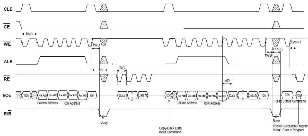
Figure 18 : Copy Back read with optional data readout /Copy back program with optional data input
