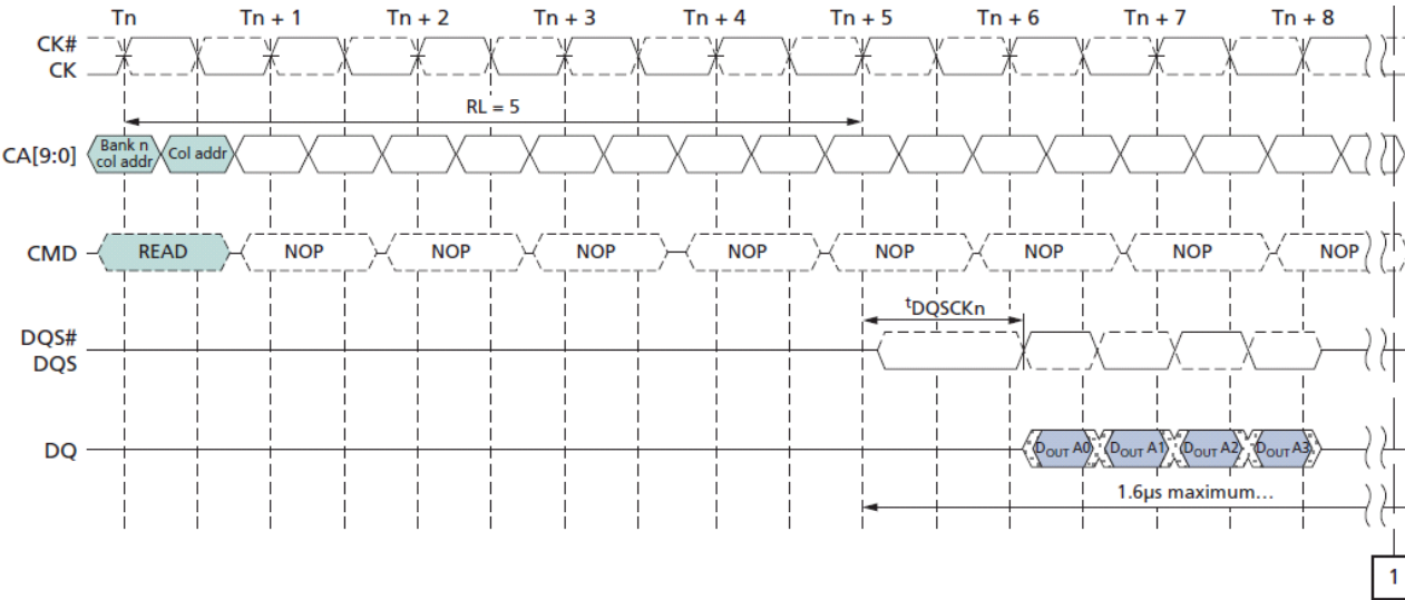
Figure 9 : tDQSCKDM Timing
