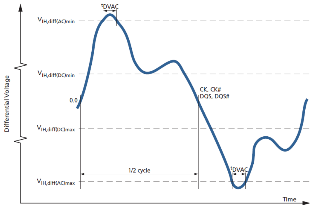
Figure 59: Differential AC Swing Time and tDVAC
