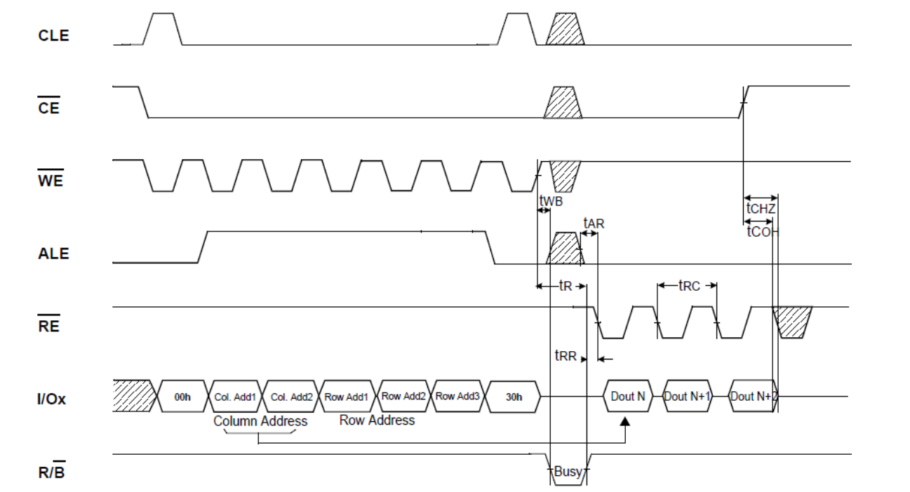
Figure 11 : Read Operation intercepted by CE#
