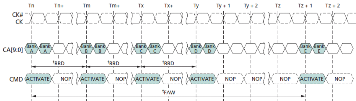
Figure 3 : tFAW Timing (8-Bank Devices)
