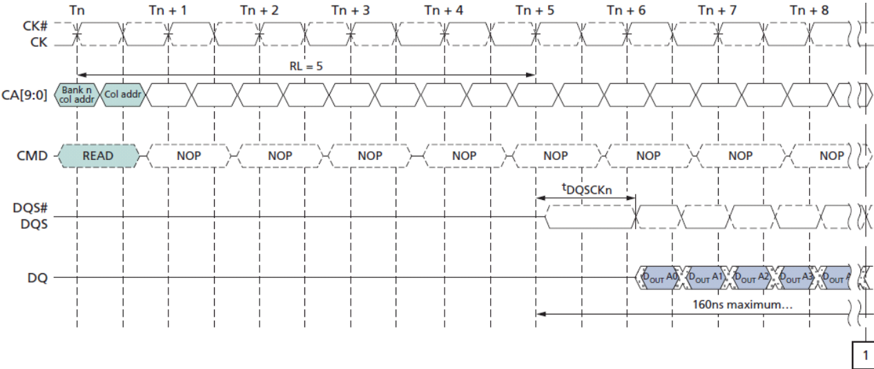
Figure 10 : tDQCKDS Timing
