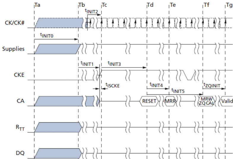
Figure 1 : Voltage Ramp and Initialization Sequence
