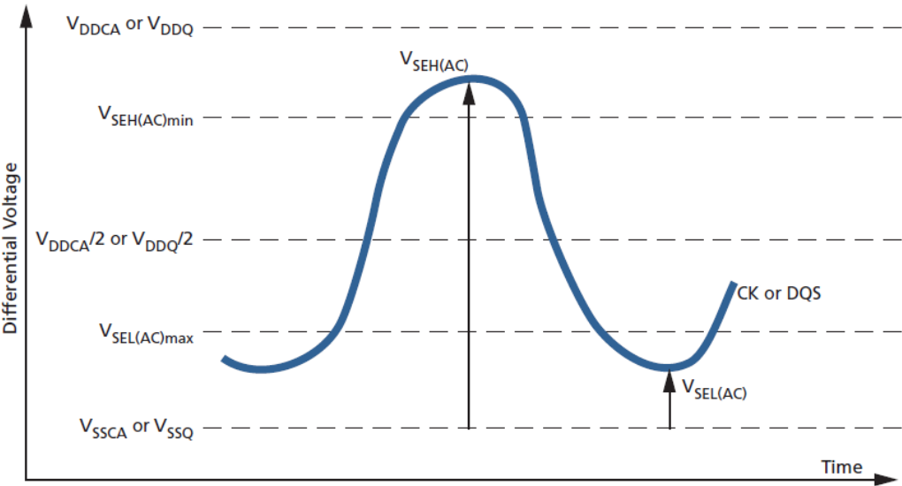
Figure 60: Single-Ended Requirements for Differential Signals
