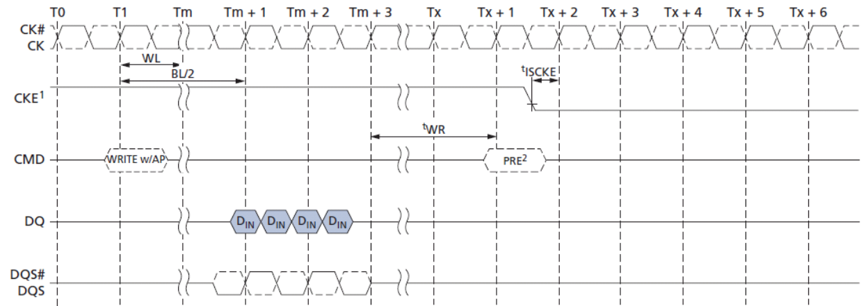
Figure 49: WRITE with Auto Precharge to Power-Down Entry
