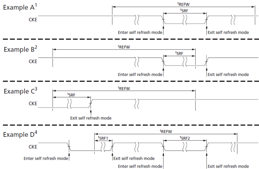
Figure 32: tSRF Definition
