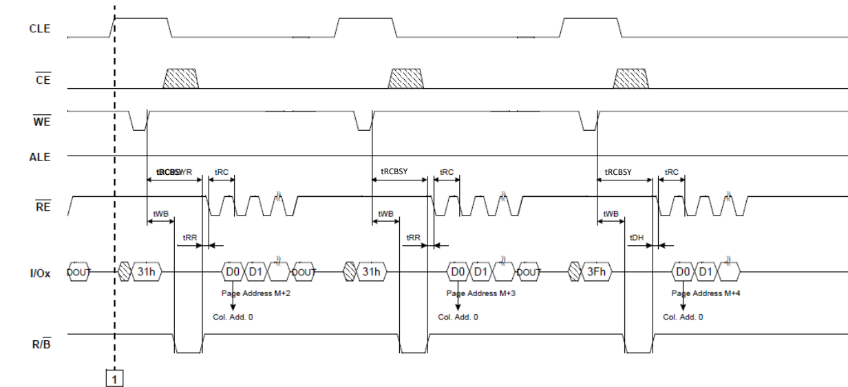
Figure 14 : read cache timings, end of cache operation
