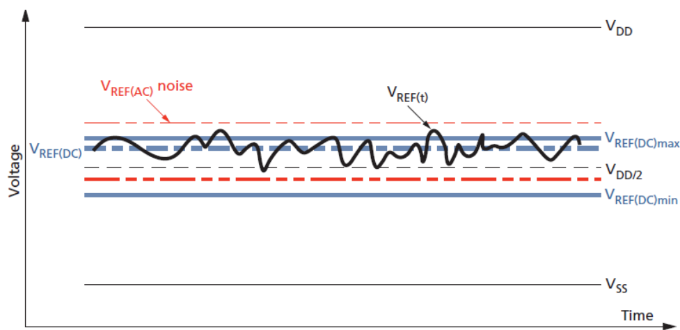
Figure 56: VREF DC Tolerance and VREF AC Noise Limits
