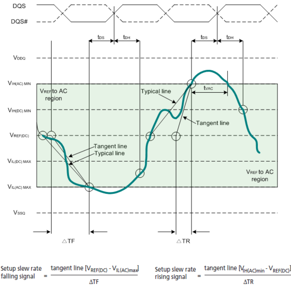
Figure 77: Tangent Line – tDS for DQ with Respect to Strobe
