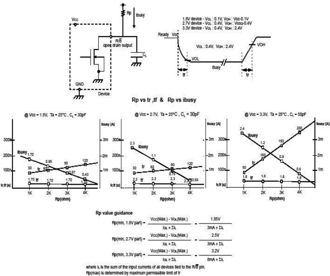
Figure 32 : Ready/Busy Pin electrical application
