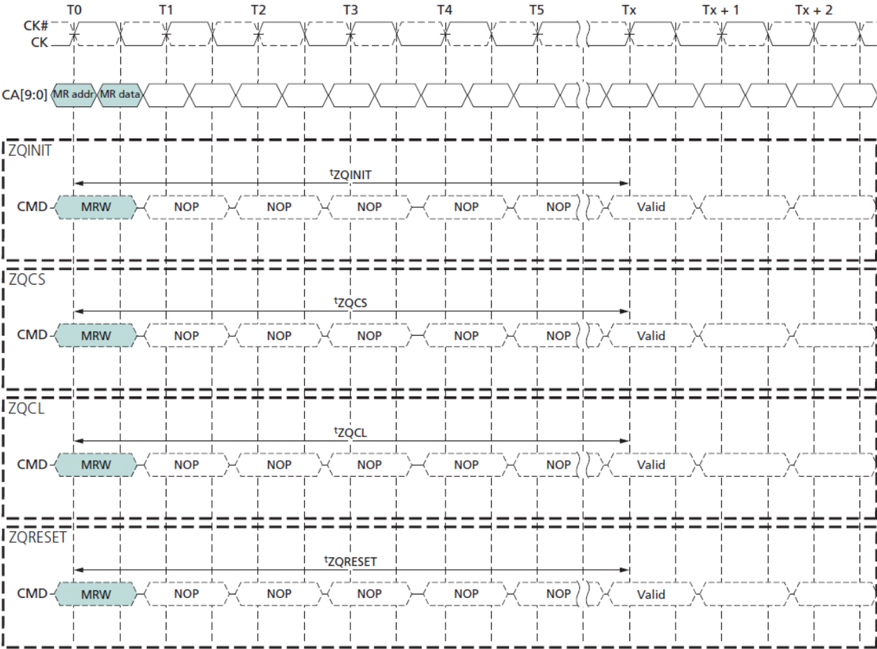
Figure 42: ZQ Timings
