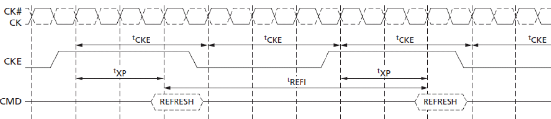
Figure 45: REFRESH-to-REFRESH Timing in CKE Intensive Environments
