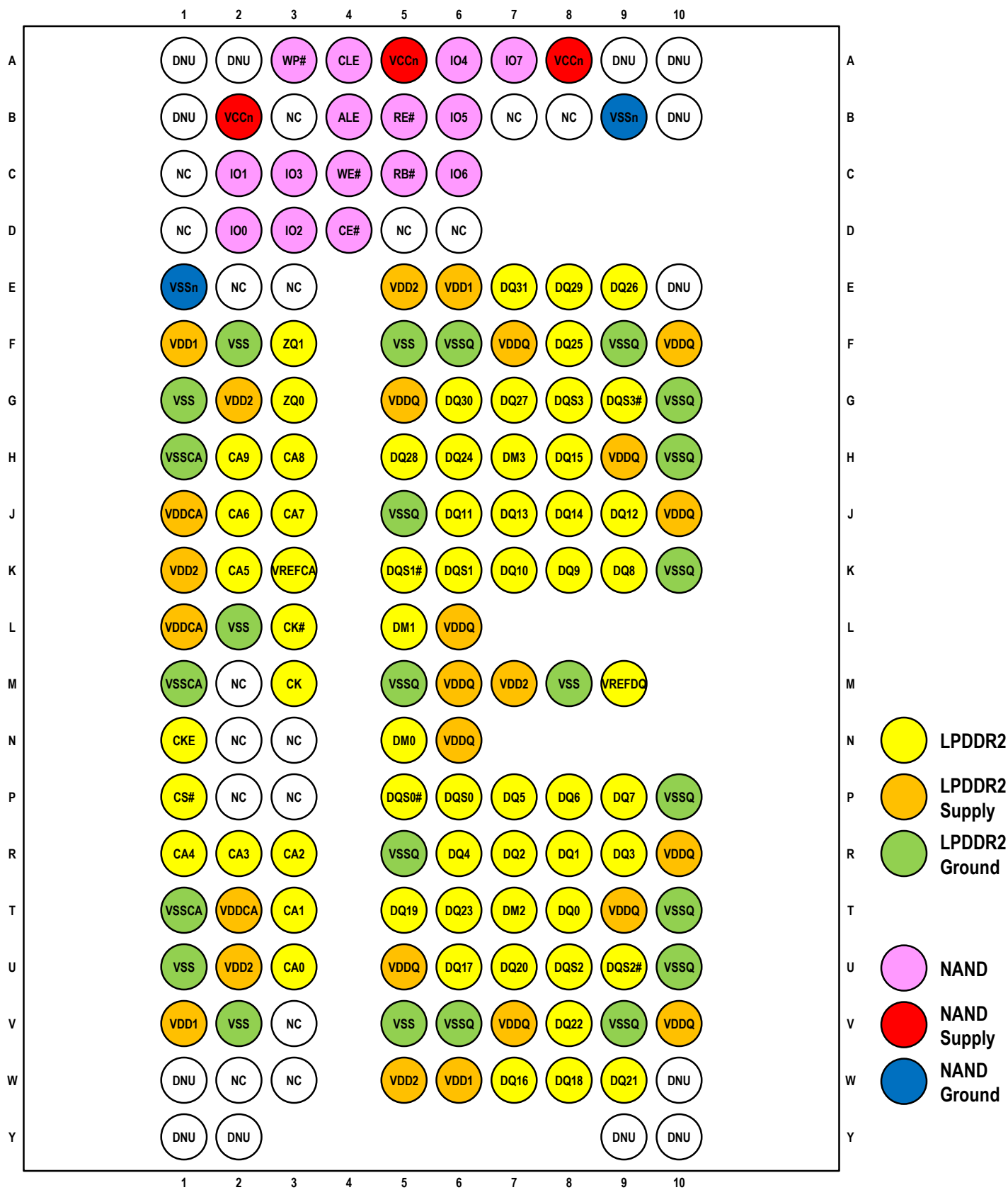
Pin Configuration – 162Ball MCP(X8/X32)
