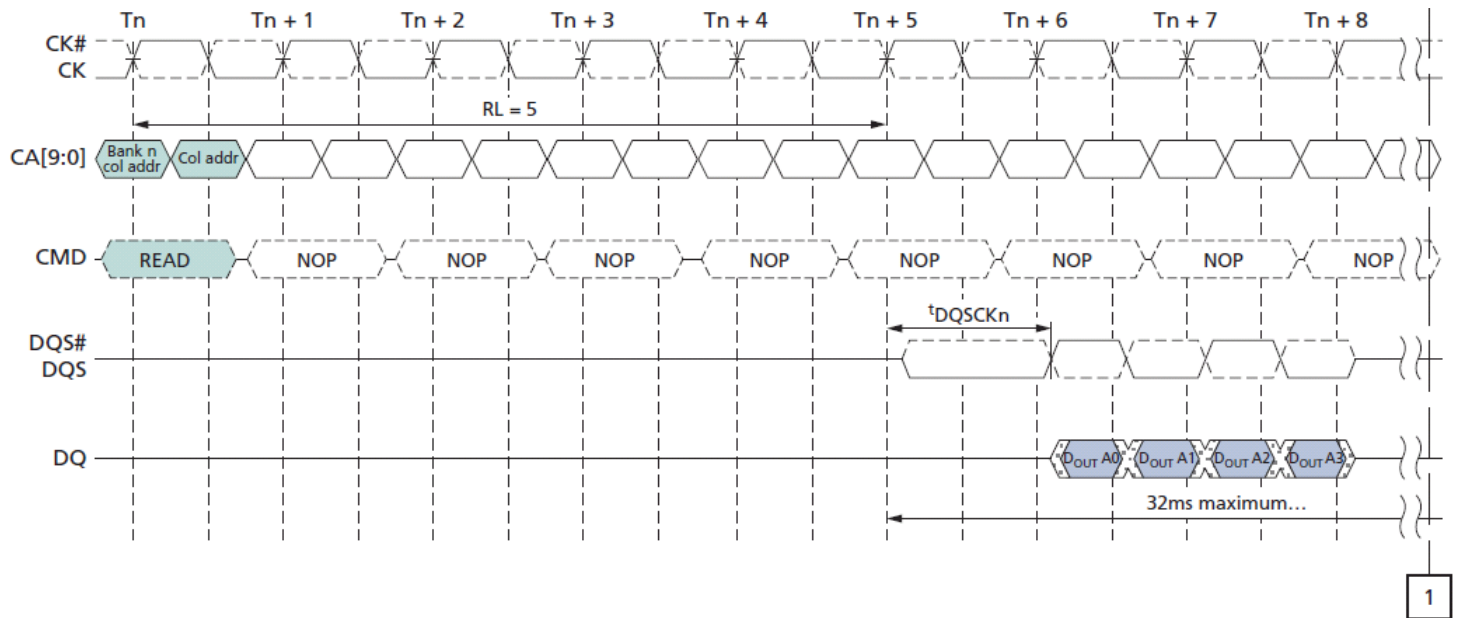
Figure 8 : tDQSKDL Timing
