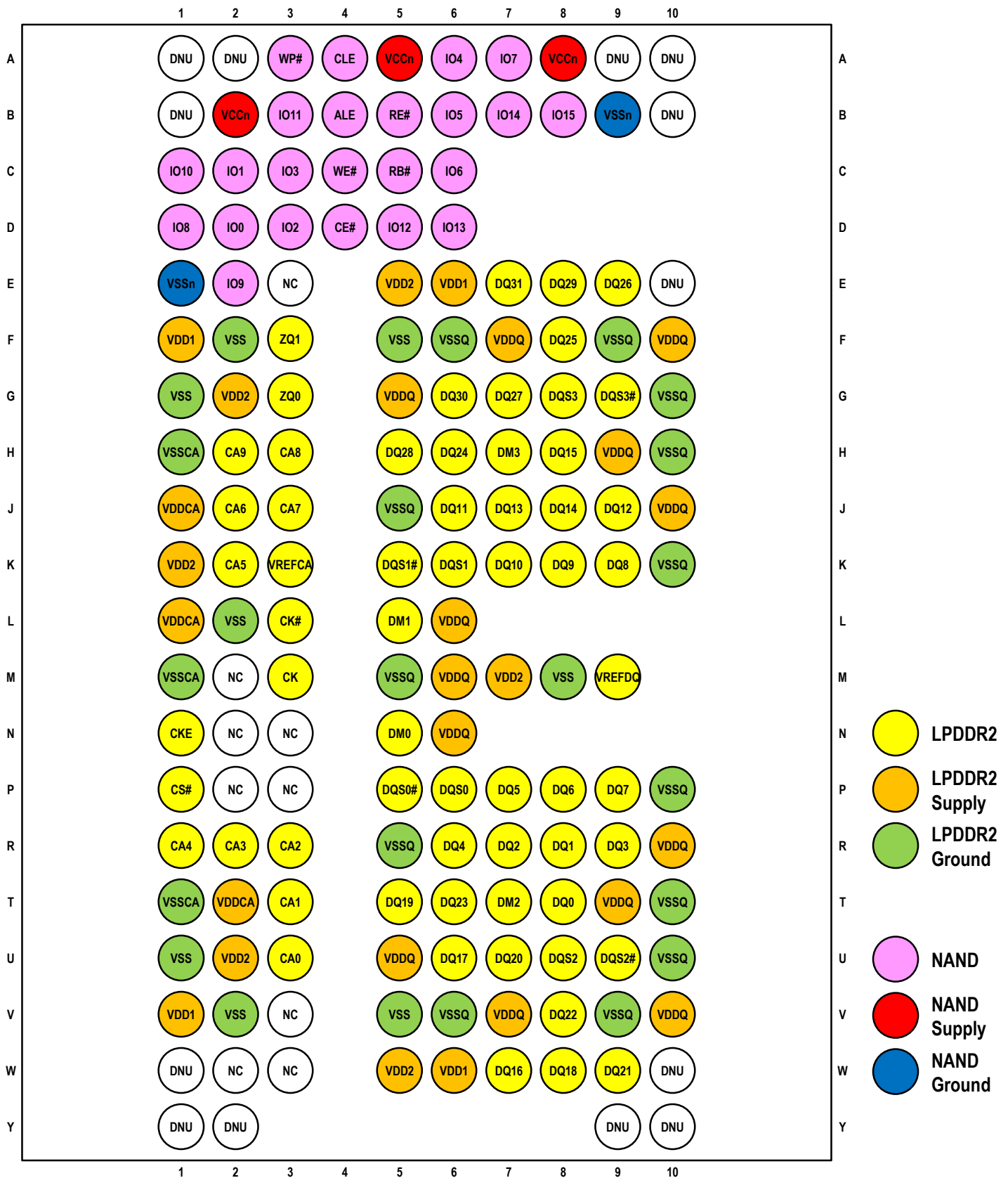
Pin Configuration – 162Ball MCP(X16/X32)
