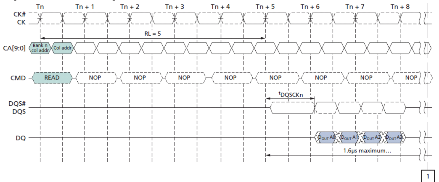
Figure 9 : tDQCKDM Timing
