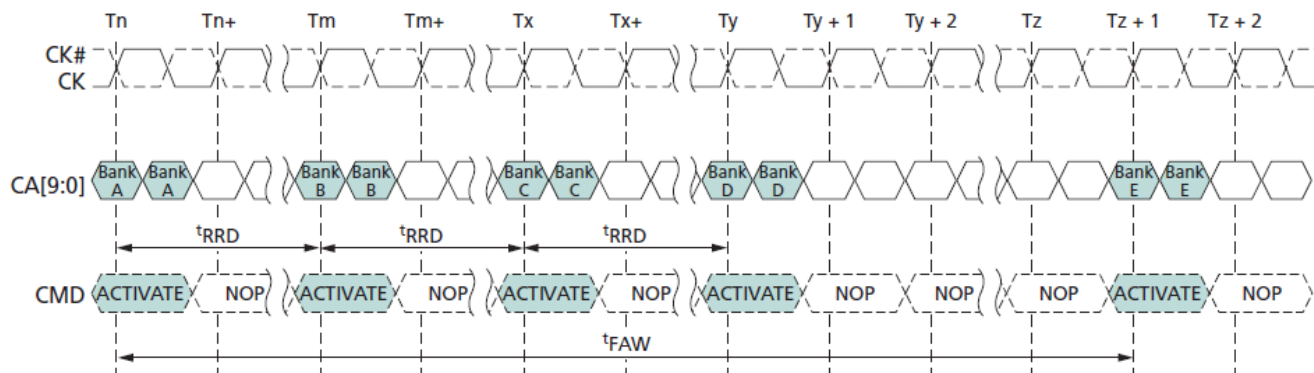
Figure 3 : tFAW Timing (8-Bank Devices)
