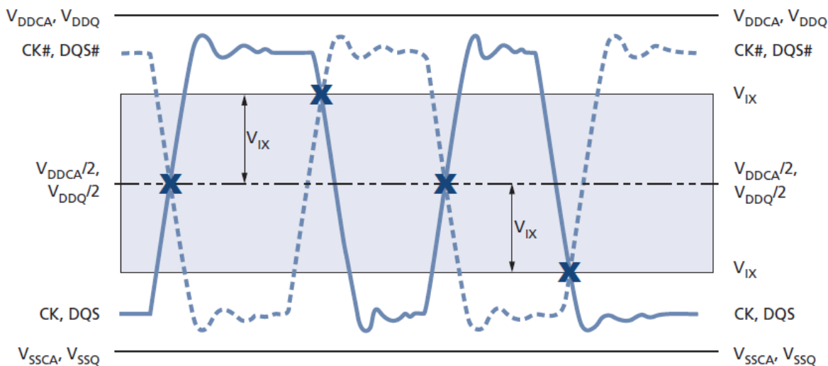
Figure 61: V_{IX} Definition
