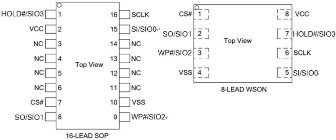
Figure 6.1 Pin Configuration
