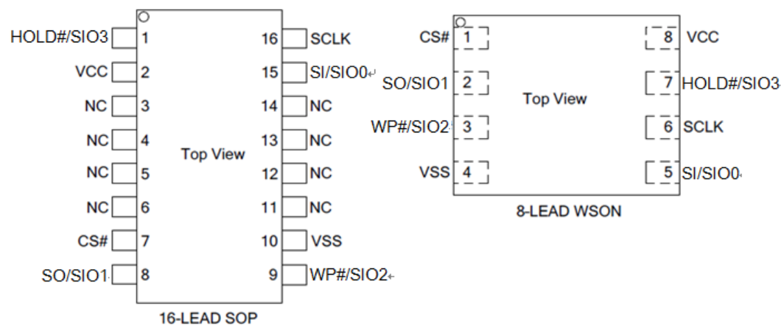
Figure 6.1 Pin Configuration
