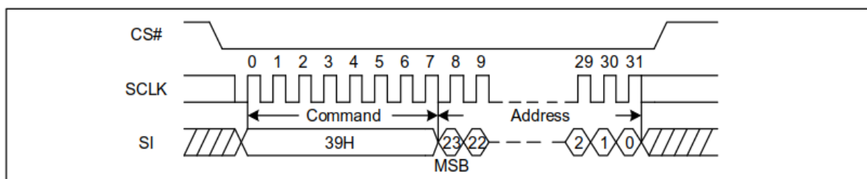
Figure 43c Individual Block/Sector Unlock command Sequence Diagram (SPI)
