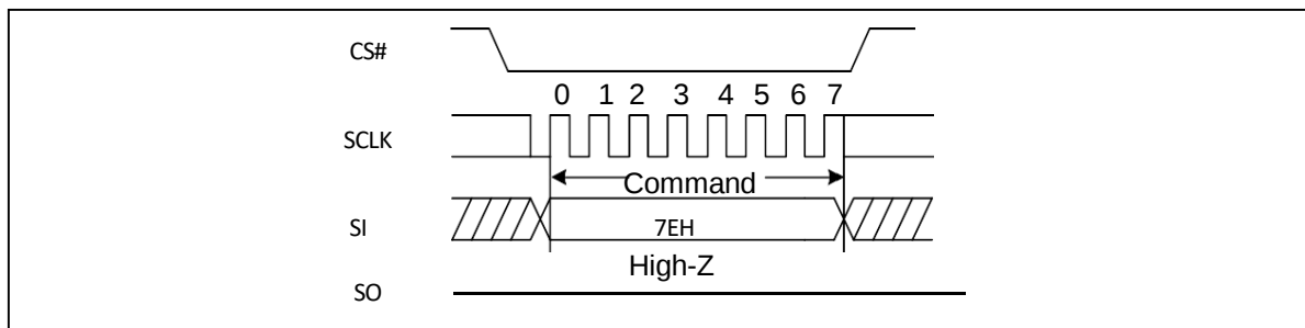
Figure 44a Global Block/Sector Lock Sequence Diagram (SPI)
